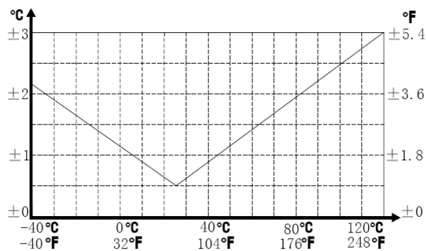
Figure 2 Temperature Accuracy
